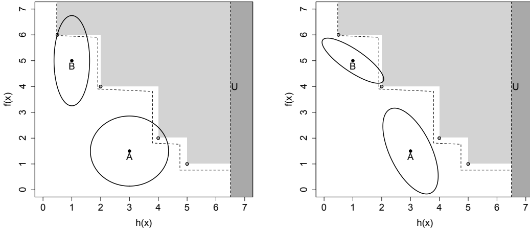
Figure 4: The probability acceptable to the filter subproblem. Selecting between candidate points A and B is determined by finding the area of their respective ellipses to the left of the filter envelope. Modeling the objective and constraint functions jointly (right) can lead to probability ellipses that are non-axis aligned as compared to independently (left) which are always axis aligned.
