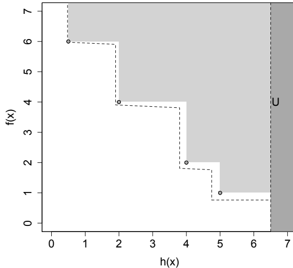
Figure 2: A typical filter. All pairs (h(\mathbf{x}), f(\mathbf{x})) that are below and to the left of the envelope (dashed line), and to the left of U , are acceptable to the filter.
