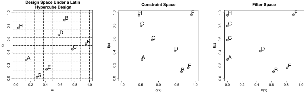
Figure 3: An example of a 2-D design space (left) where eight points were sampled using a Latin hypercube design. Also, an example of the constraint space ( c(\mathbf{x}) , f(\mathbf{x}) ) (center) and the mapping to the filter space ( h(\mathbf{x}) , f(\mathbf{x}) ) (right). Points in the constraint space such that c(\mathbf{x}) \leq 0 get mapped to h(\mathbf{x}) = 0 in the filter space.
