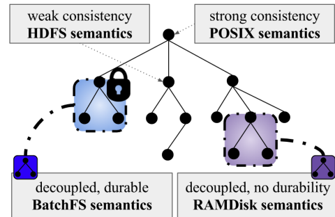
Fig. 1: Illustration of subtrees with different semantics co-existing in a global namespace. For performance, clients relax consistency/durability on their subtree ( e.g. , HDFS) or decouple the subtree and move it locally ( e.g. , BatchFS, RAMDisk).
