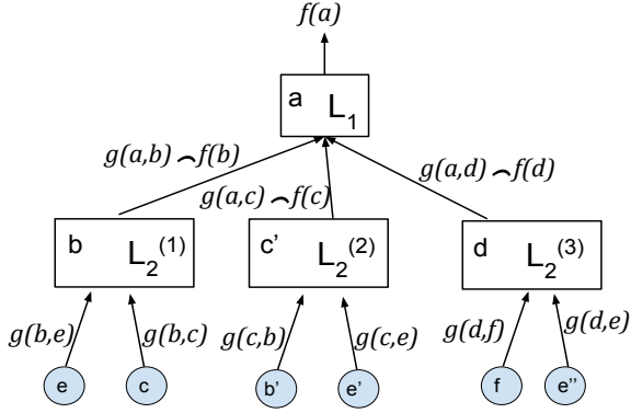
Figure 2: Forward propagation corresponding to the tree unfolding of Figure 1. The elements of the sequence which is fed to learner L_1 consist of the features of the respective edges concatenated with the output from learners below. Note the use of three instances of the learner L_2 , one for each depth-2 node in the unfolding. These instances share the same parameters. In the figure, the symbol \sim denotes the concatenation of feature vectors.
