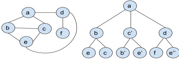
Figure 1: An example of a graph and its asymmetric unfolding at node a for depth 2. We rename the nodes that appear in many locations so that they have distinct names, for instance, we use e , e' and e'' to denote the copies of e .
