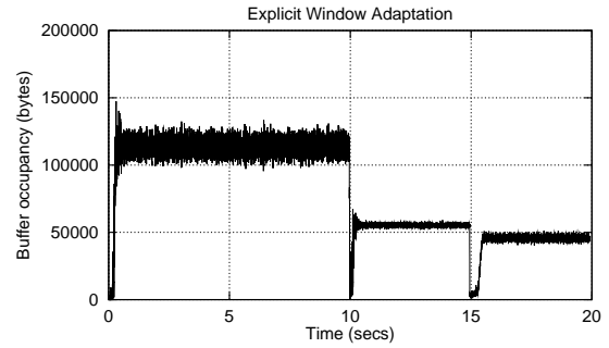
Figure 4.10: Buffer size at IP-ATM Router 1 with EWA (IP Network 1 delays vary from 1 to 5 msecs, ATM backbone delay = 5 msecs).
