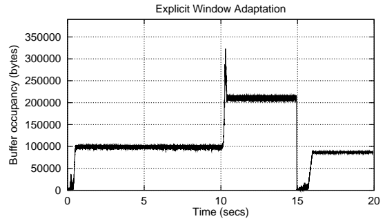
Figure 4.14: Buffer size at IP-ATM Router 1 with EWA (IP Network 1 delays = 5 msec, ATM backbone delay = 5 msec).
