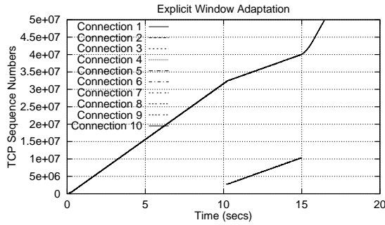
Figure 4.13: Sequence number growth for TCP connections with EWA (IP Network 1 delays = 5 msec, ATM backbone delay = 5 msec).
