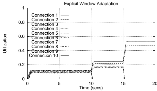
Figure 4.11: Utilization for each individual connection at link L1 with EWA measured in intervals of 250 msecs (IP Network 1 delays vary from 1 to 5 msecs, ATM backbone delay = 5 msecs).
