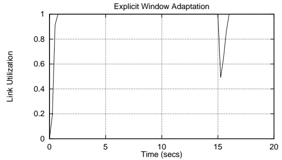
Figure 4.16: Effective utilization of the ATM link at IP-ATM Router 1 with EWA measured in intervals of 250 msec (IP Network 1 delays = 5 msec, ATM backbone delay = 5 msec).
