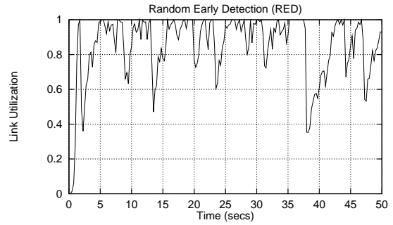
Figure 4.26: Effective utilization of the ATM link at IP-ATM Router 1 with RED measured in intervals of 250 msec (in total there are 10 persistent TCP sources, 30 ON-OFF TCP sources with mean ON-time = mean OFF-time = 200 ms, max_p = 0.05 , min_{th} = 150 , max_{th} = 400 , IP Network 1 delays = 49 msec, ATM backbone delay = 1 msec).
