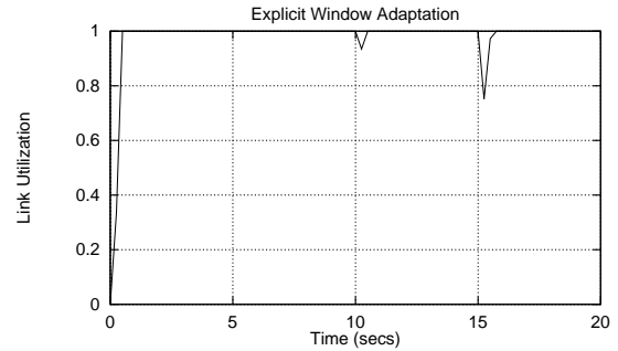
Figure 4.12: Effective utilization of the ATM link at IP-ATM Router 1 with EWA measured in intervals of 250 msecs (IP Network 1 delays vary from 1 to 5 msecs, ATM backbone delay = 5 msecs).
