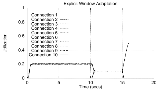
Figure 4.15: Utilization for each individual connection at link L1 with EWA measured in intervals of 250 msec (IP Network 1 delays = 5 msec, ATM backbone delay = 5 msec).
