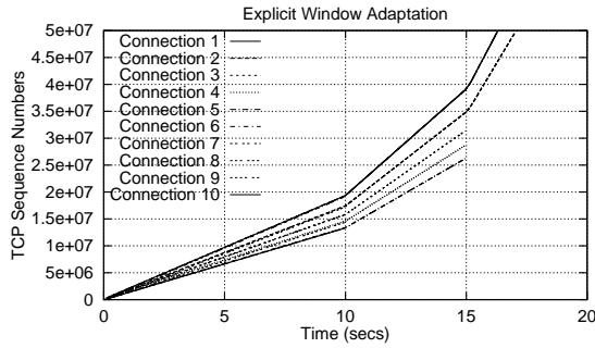
Figure 4.9: Sequence number growth for TCP connections with EWA (IP Network 1 delays vary from 1 to 5 msecs, ATM backbone delay = 5 msecs).
