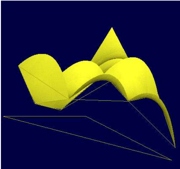
Figure 12: IFS surface interpolation of scattered data.
