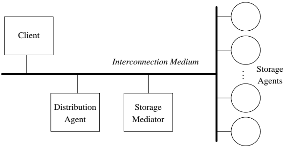
Figure 1: Components of the Swift Architecture
