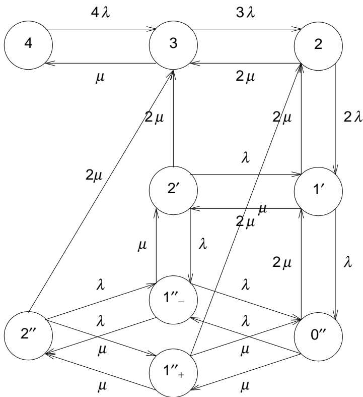
Figure 4: RDV State Transition Diagram for Four Replicas
