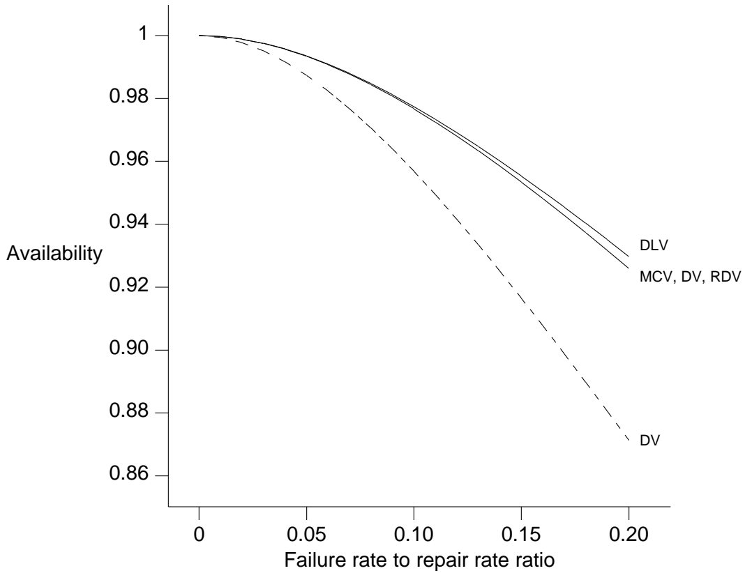
Figure 6: Compared Availabilities for Three Replicas
