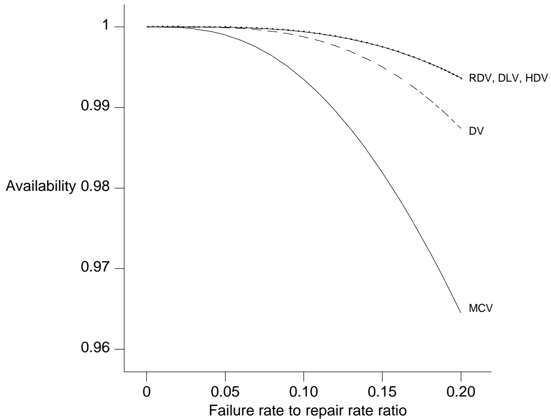
Figure 8: Compared Availabilities for Five Replicas
