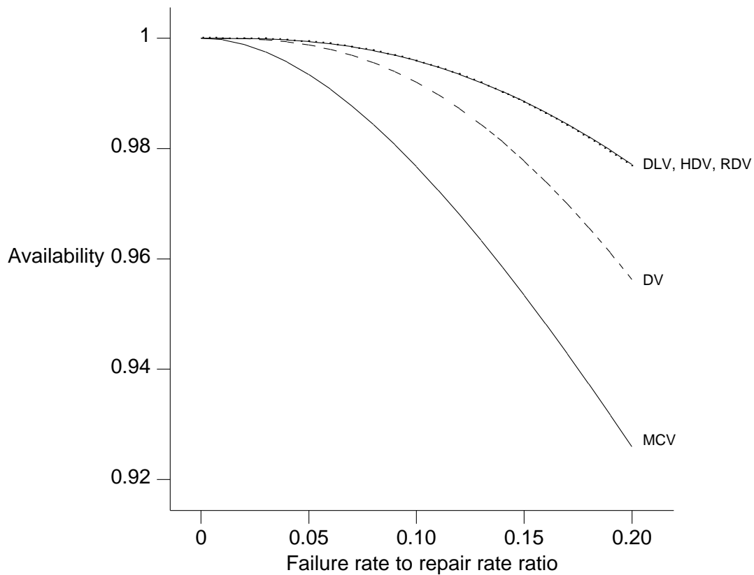
Figure 7: Compared Availabilities for Four Replicas
