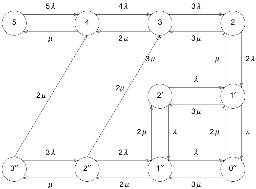
Figure 5: RDV State Transition Diagram for Five Replicas
