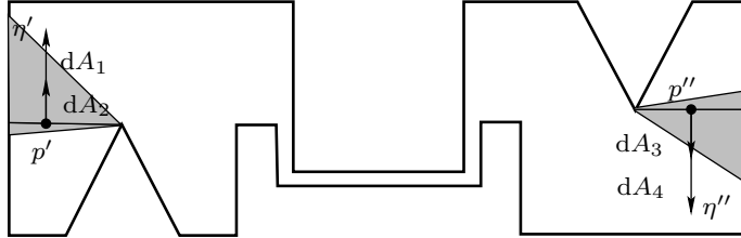
FIG. 2.6. Example polygon for which A \circ S and -A \circ S restricted to Q \setminus \text{Ver}_r(Q) are not regular. Note here that dA_1 and dA_2 are not perfectly aligned with \eta' . Also, dA_3 and dA_4 are not perfectly aligned with \eta'' .
